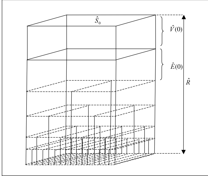
FIGURE 3. The straightened tree, \hat{T}_3 for k = 3, N = 3 .
